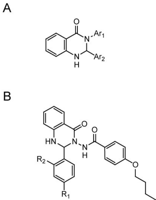
Fig. 1. Chemical structure of the core compound and Quin-C1. A, the core structure based on which Quin-C1 is developed. B, the structure of Quin-C1 (4-butoxy-N-[2-(4-methoxy-phenyl)-4-oxo-1,4-dihydro-2H-quinazolin-3-yl]-benzamide), in which R 1 = -OCH 3 , and R 2 = H.
